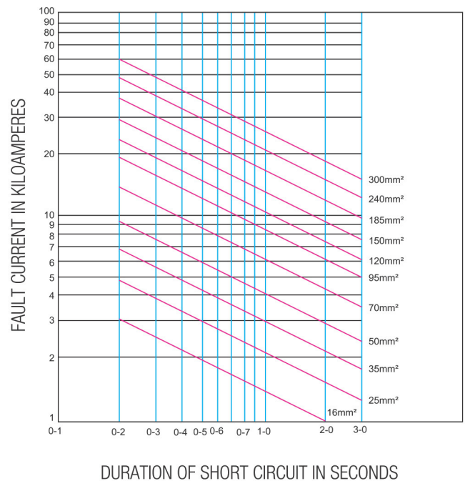
ALUMINIUM CONDUCTORS
