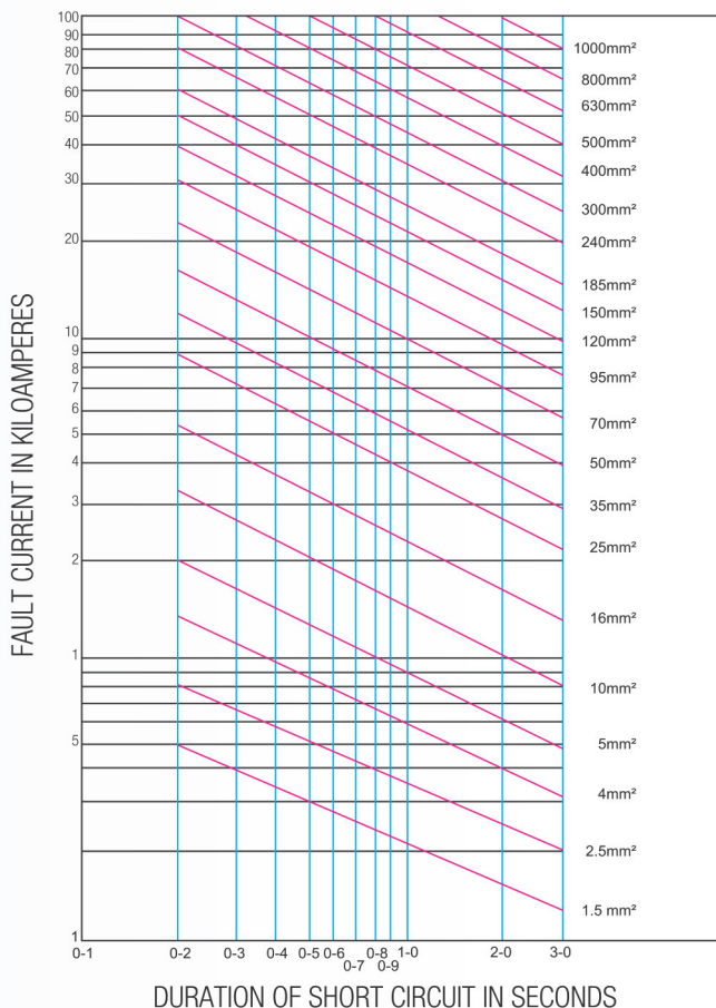
COPPER CONDUCTORS
